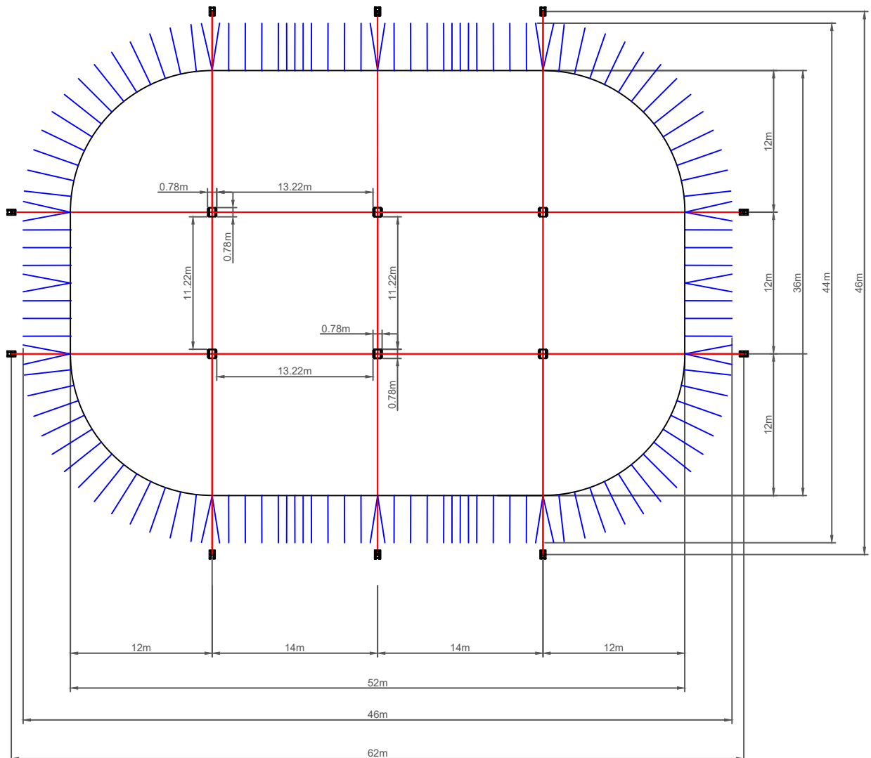
PLAN LAYOUT (NTS)
